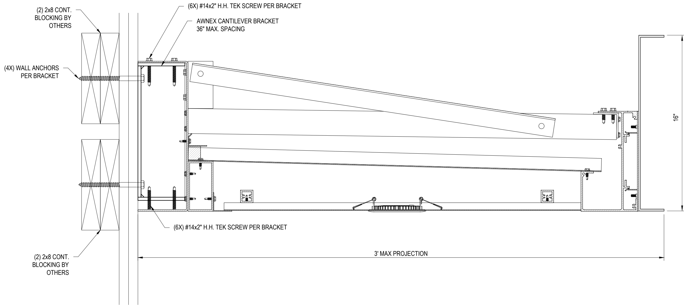
CANTILEVER COLORADO FRONT GUTTER SECTION VIEW 16" OPEN FACE
