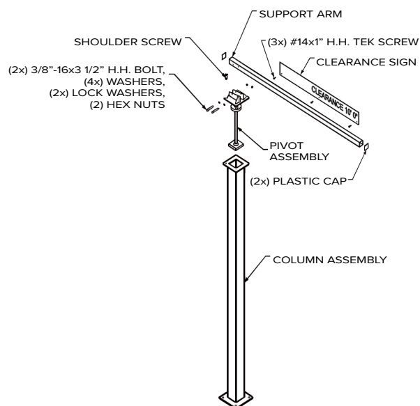
PIVOTED CLEARANCE BAR
