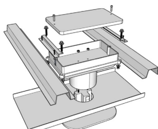
SOFFIT LIGHT INSTALL
