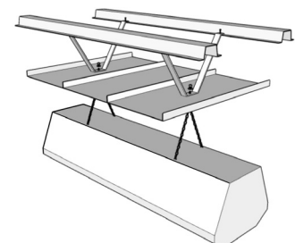
HEATER INSTALL
