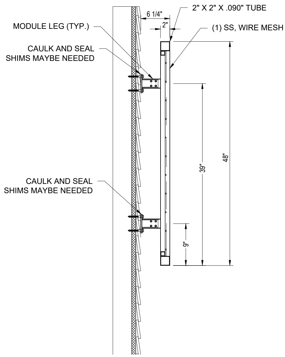
SECTION A-A SIDING WALL
