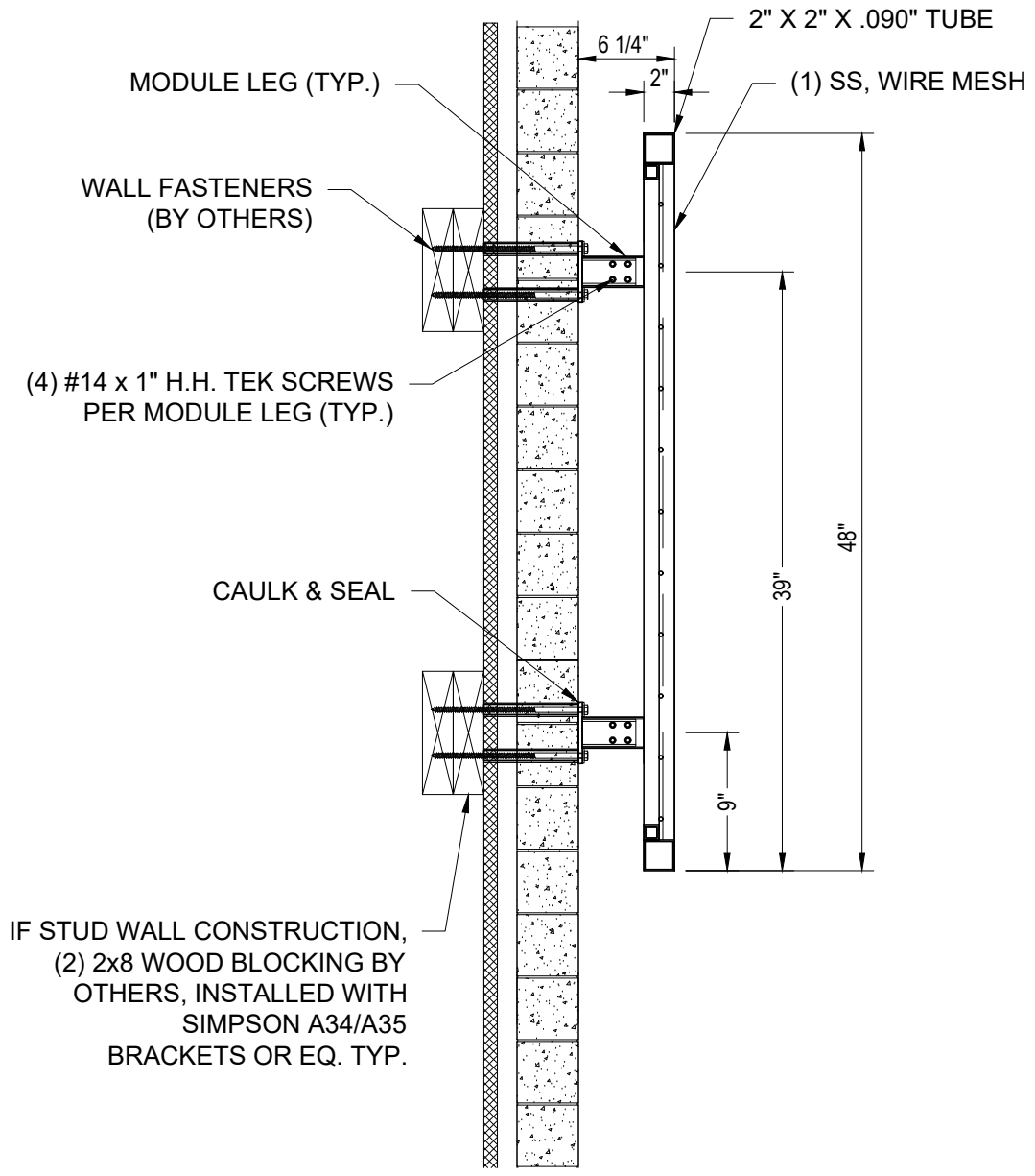
SECTION A-A BRICK WALL
