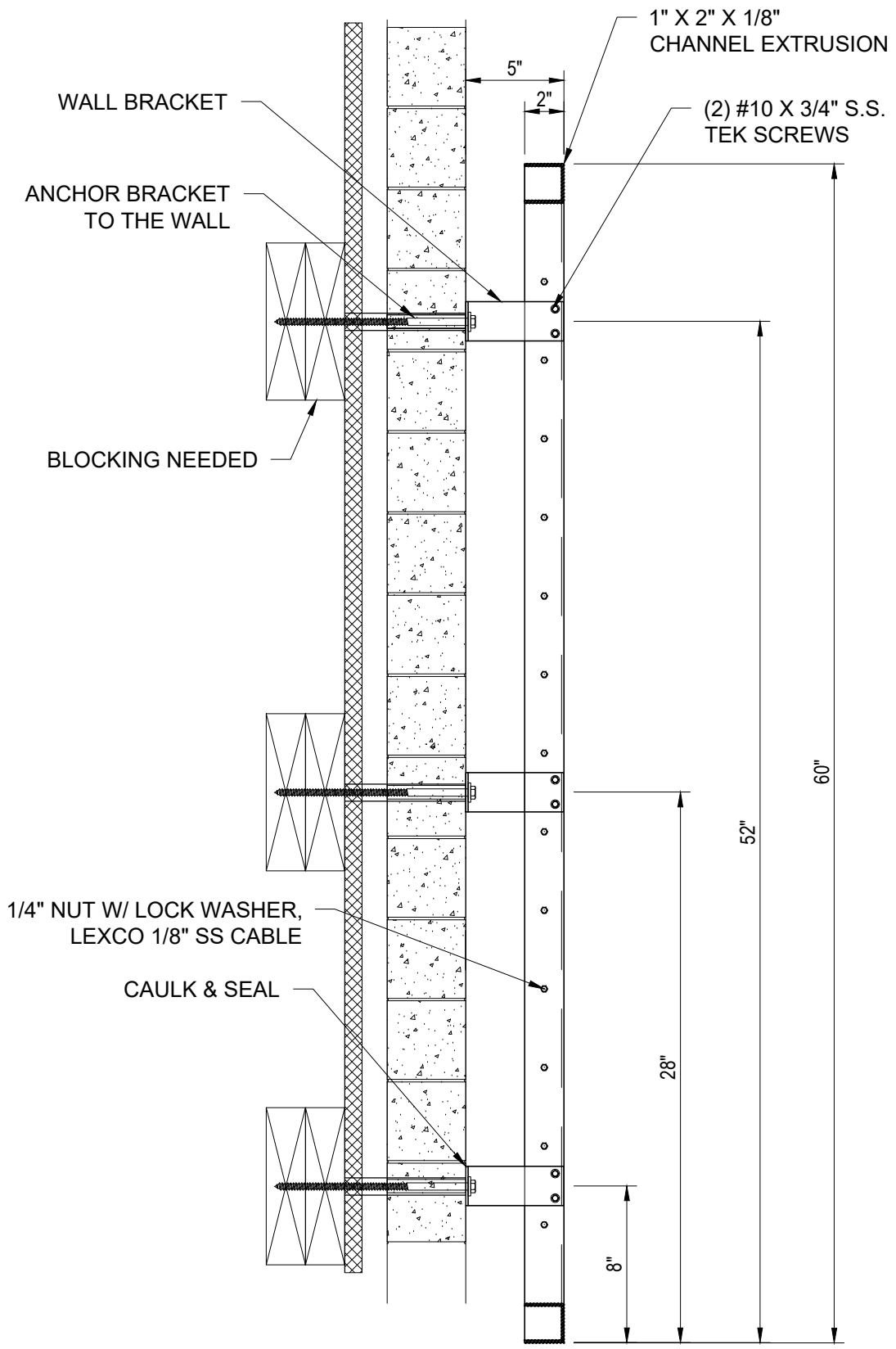
SECTION A-A BRICK WALL
