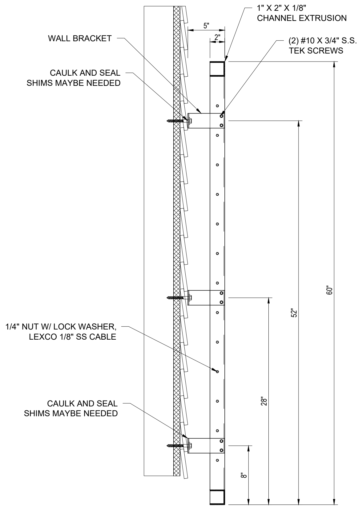
SECTION A-A SIDING WALL
