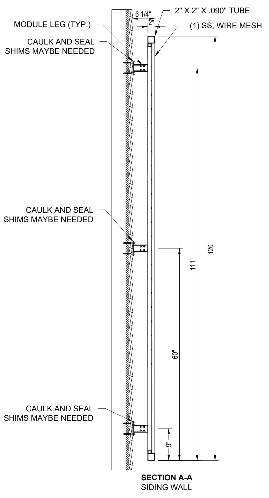
FRAME DETAIL
