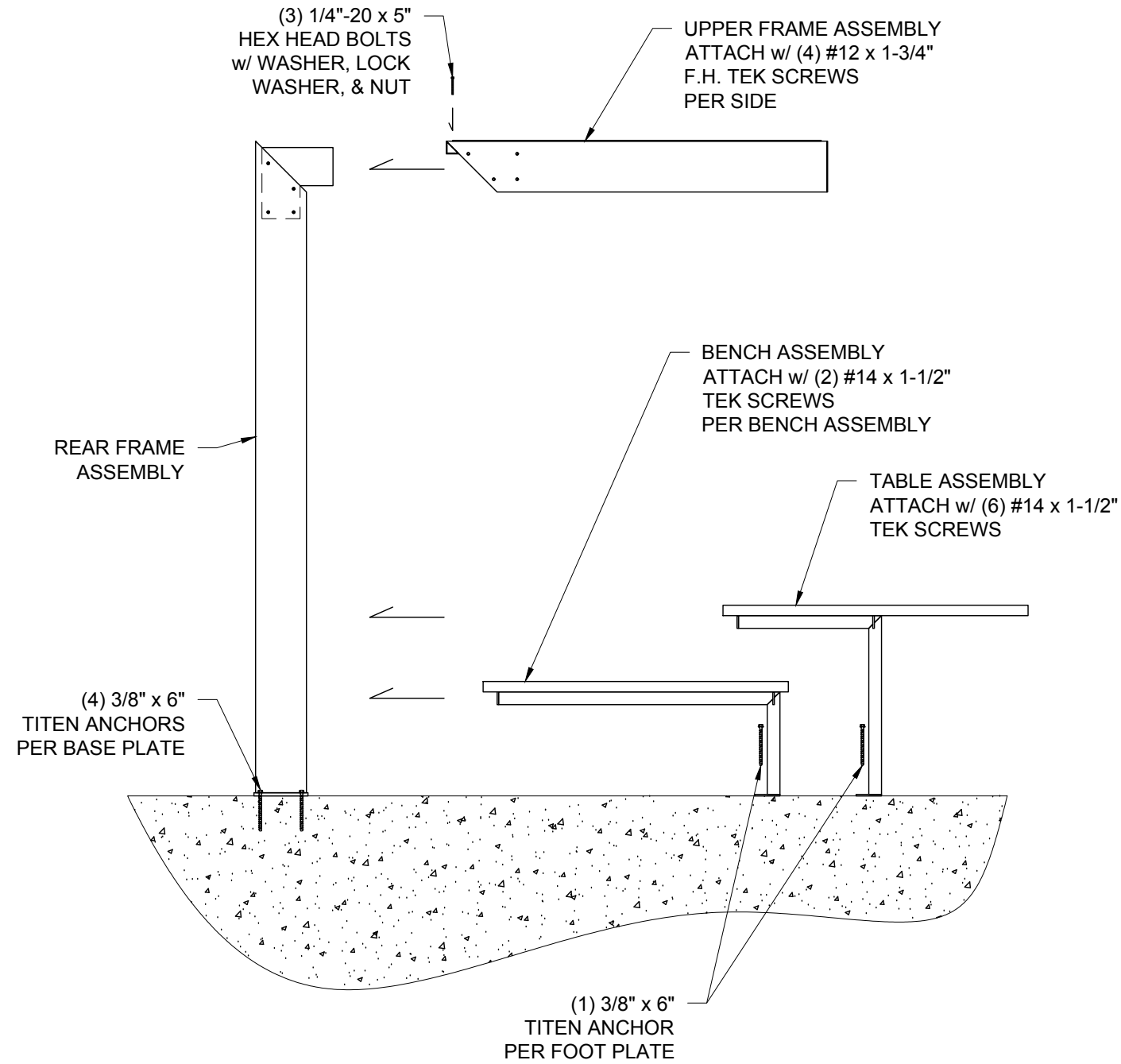
TYPICAL INSTALL
