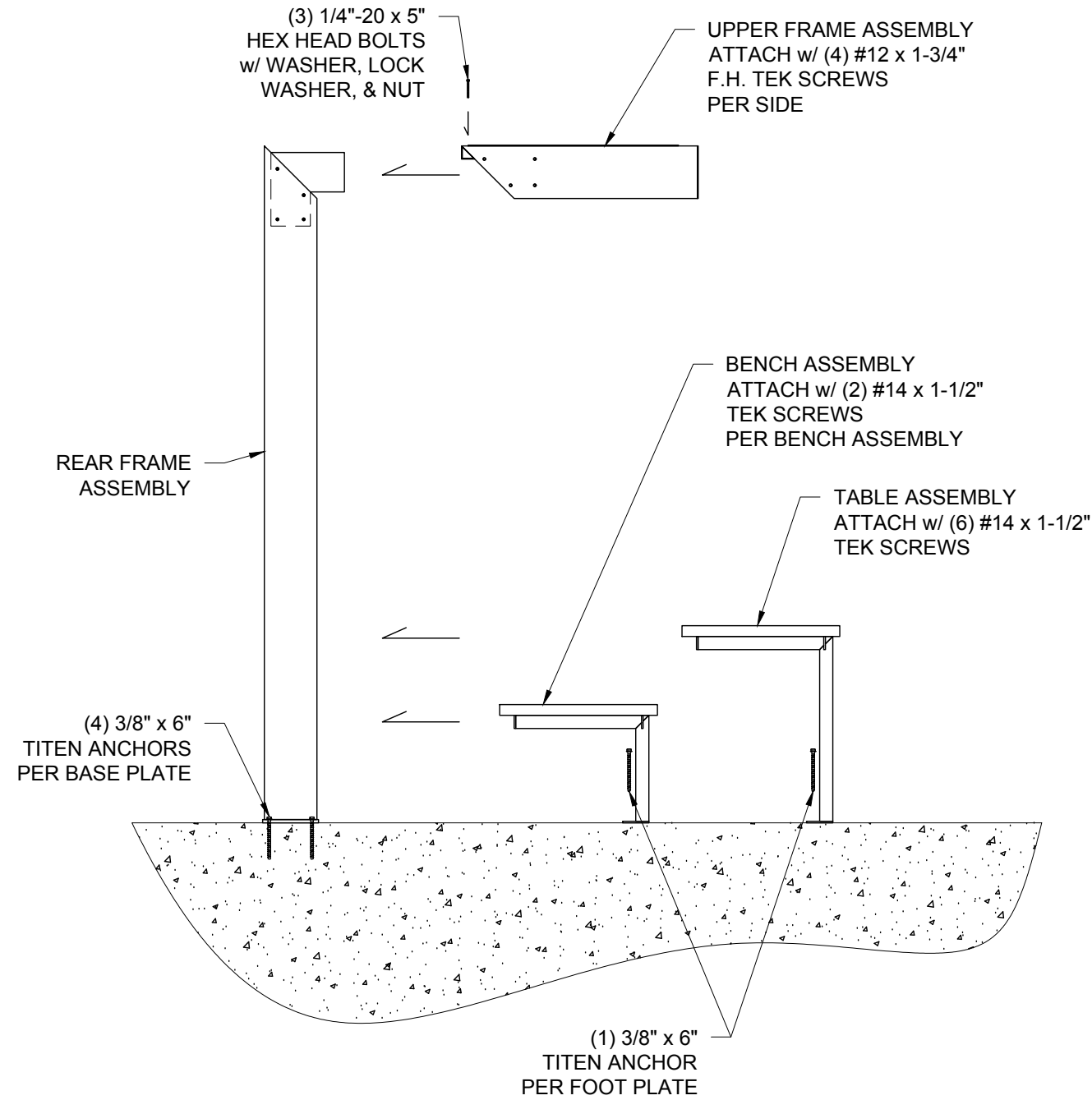
TYPICAL INSTALL
