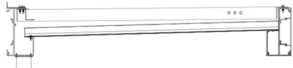
REAR GUTTER WITH OUTLET
