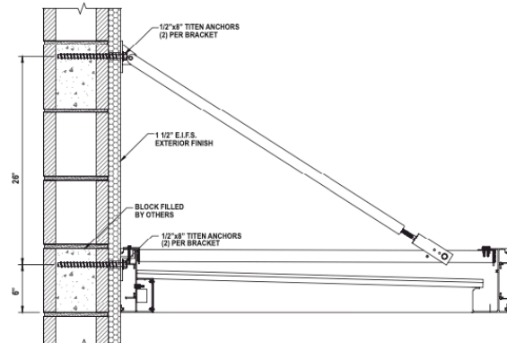
E.F.I.S OVER CMU BLOCK WALL
