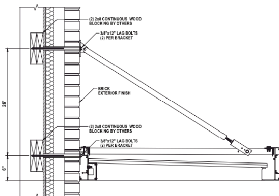
BRICK WITH INSULATION OVER WOOD BLOCKING
